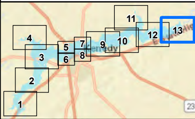
Figure C-6 FRS No. 1 and FRS No. 13 FBH Breach Inundation Map 13 of 13
