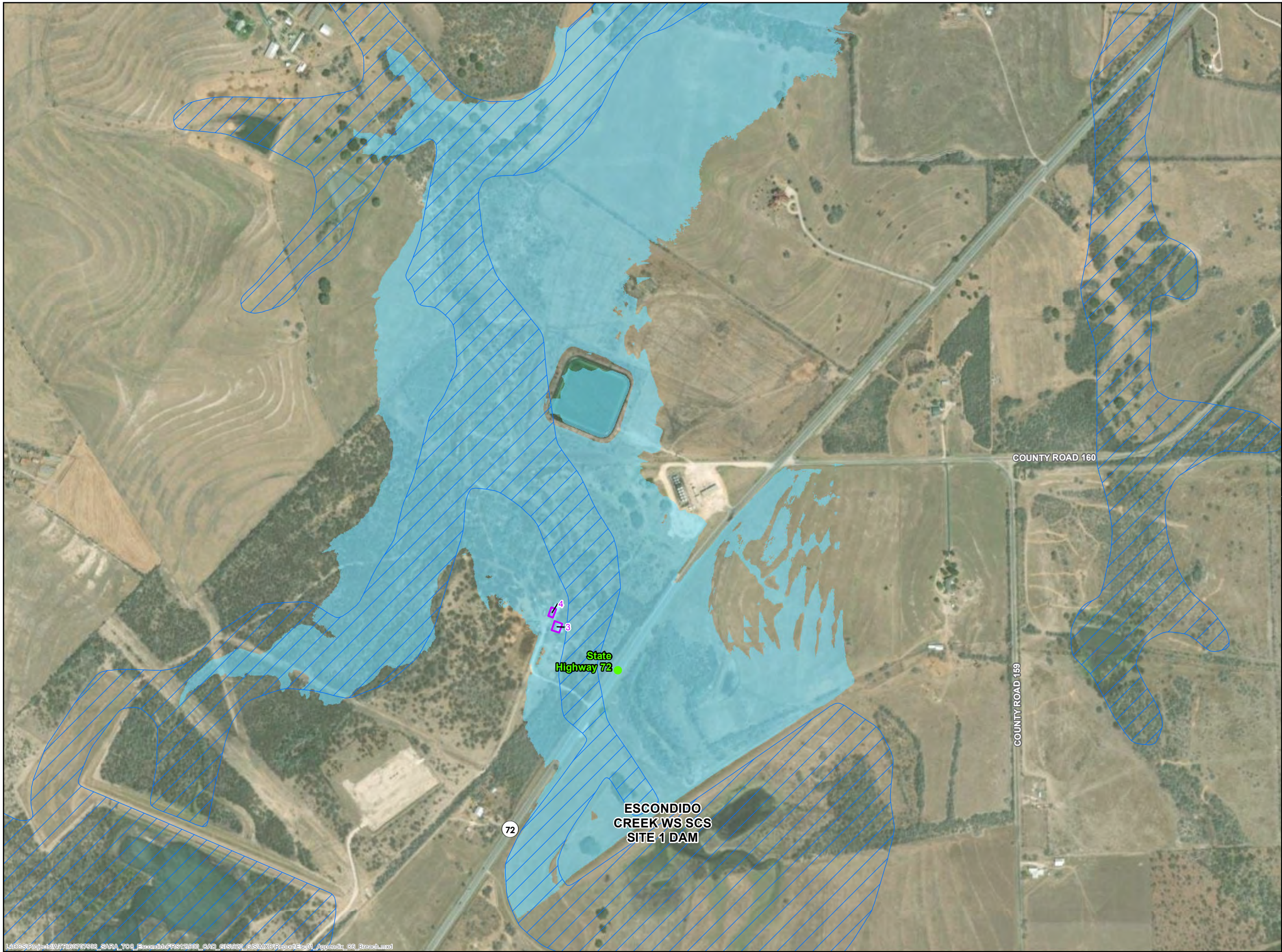
Figure C-6 FRS No. 1 and FRS No. 13 FBH Breach Inundation Map 1 of 13
