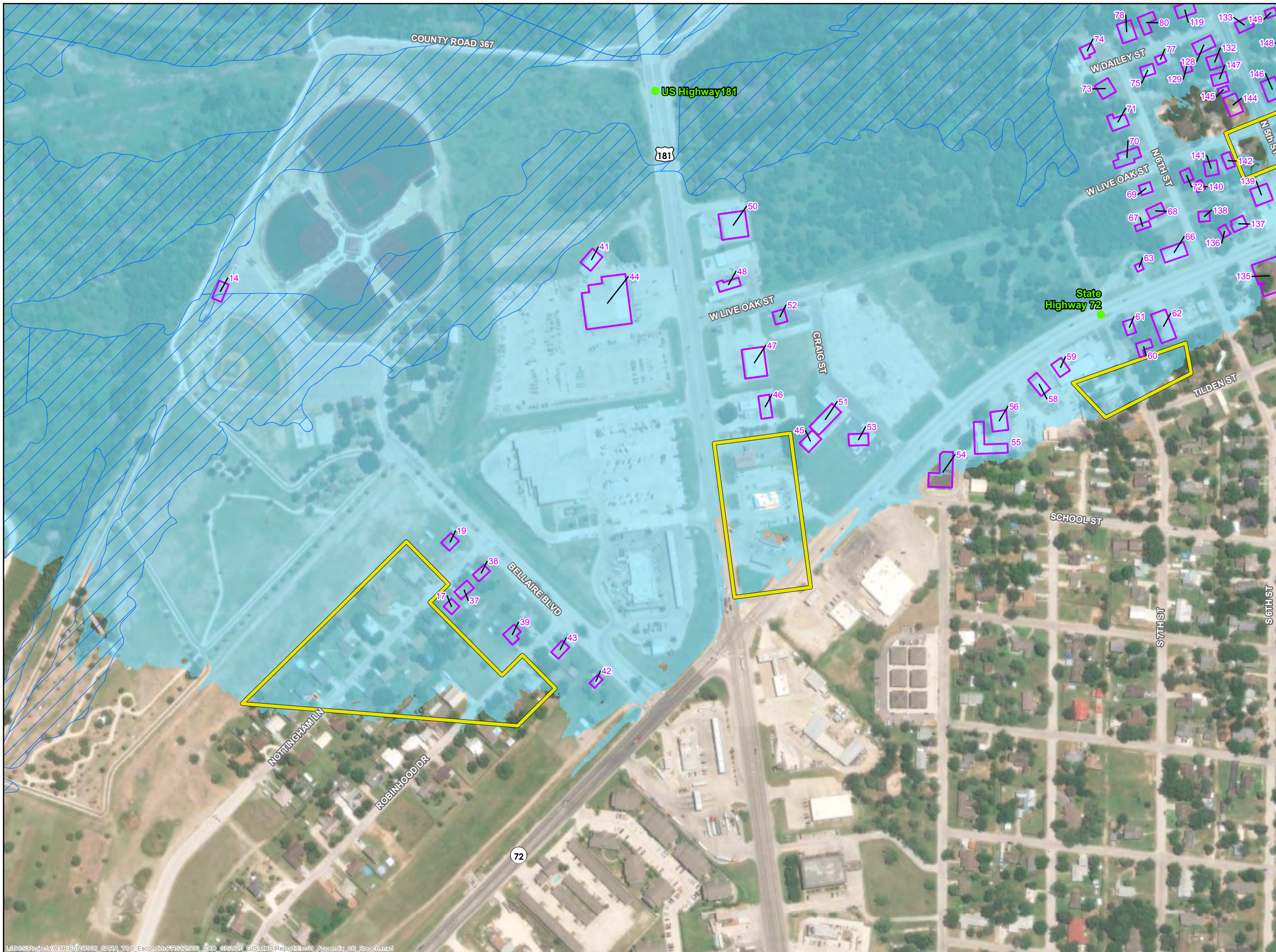
Figure C-6 FRS No. 1 and FRS No. 13 FBH Breach Inundation Map 6 of 13
