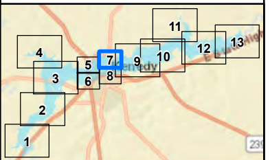
Figure C-6 FRS No. 1 and FRS No. 13 FBH Breach Inundation Map 7 of 13
