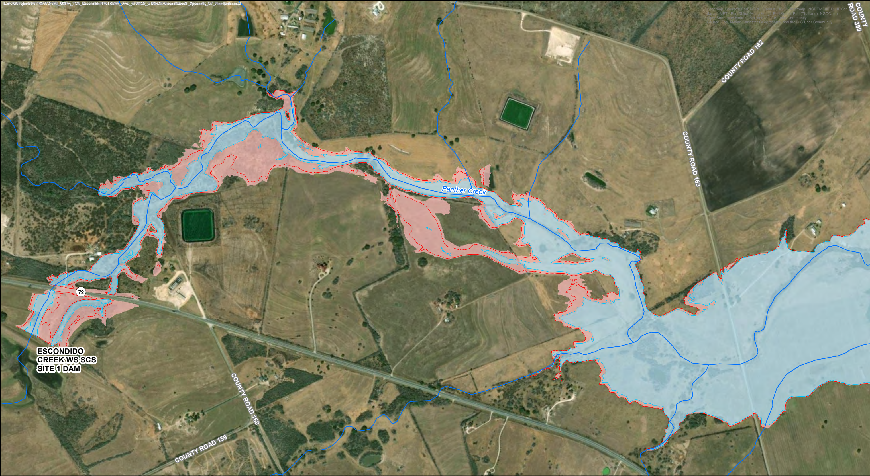
Escondido Creek Watershed Karnes County, Texas Figure C-7 FRS No. 1 Floodplain Map 1 of 6
