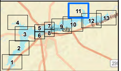
Escondido Creek Watershed FRS No. 1 Karnes County, Texas Figure C-6 FRS No. 1 and FRS No. 13 FBH Breach Inundation Map 11 of 13
