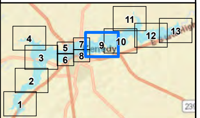
Figure C-6 FRS No. 1 and FRS No. 13 FBH Breach Inundation Map 9 of 13
