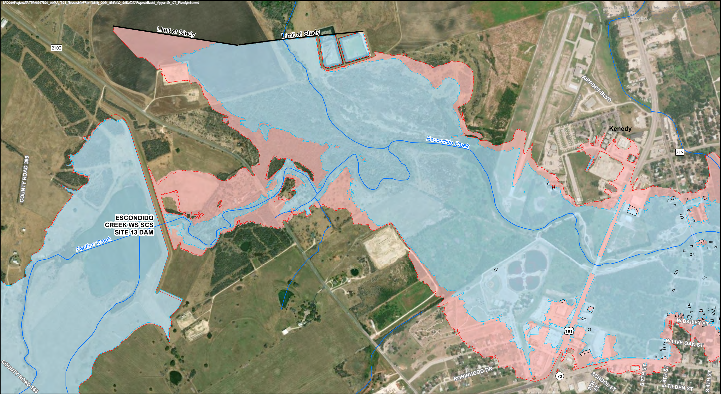
Escondido Creek Watershed Karnes County, Texas Figure C-7 FRS No. 1 Floodplain Map 2 of 6
