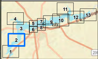
Figure C-6 FRS No. 1 and FRS No. 13 FBH Breach Inundation Map 2 of 13
