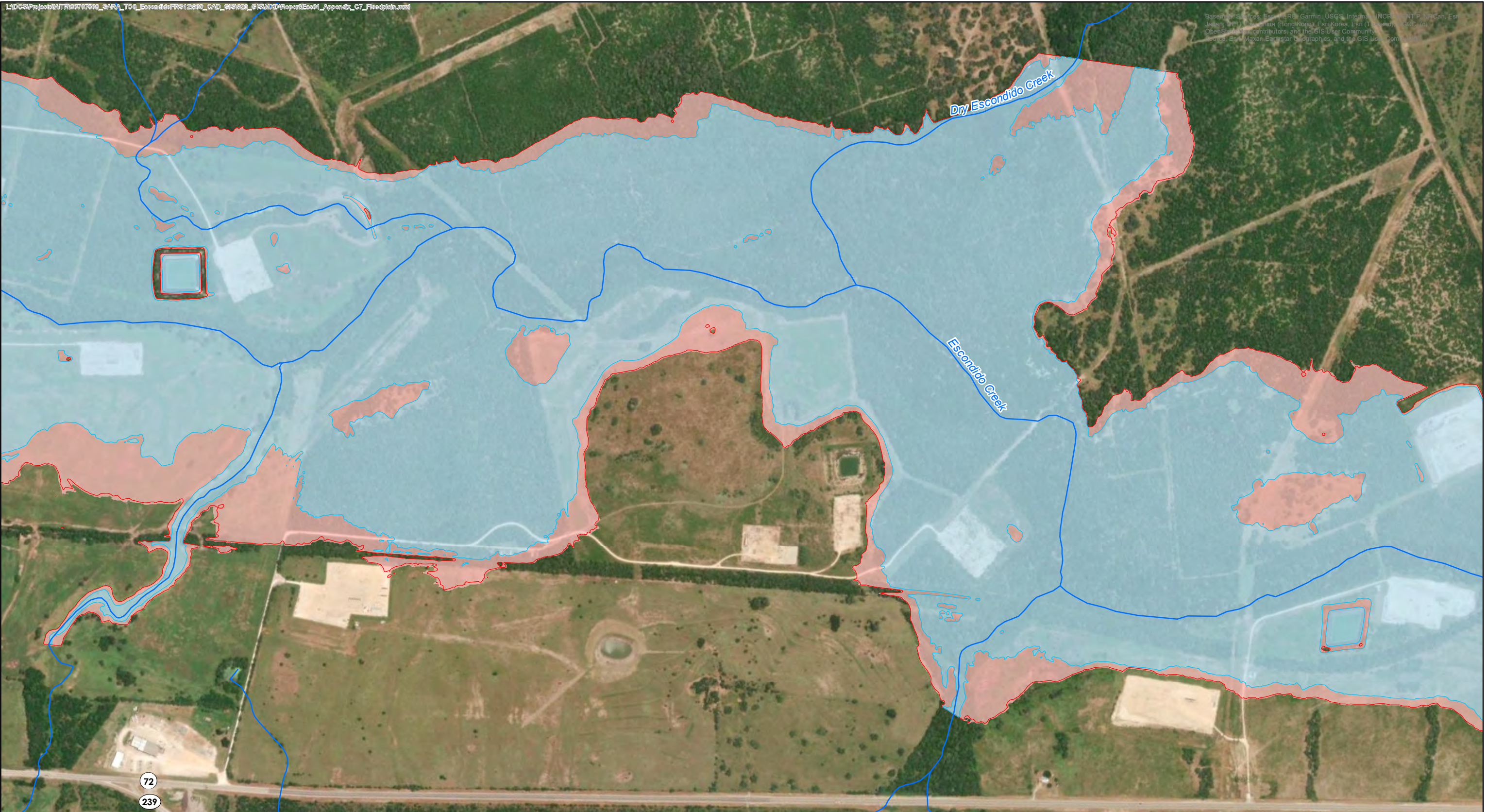
Escondido Creek Watershed Karnes County, Texas Figure C-7 FRS No. 1 Floodplain Map 4 of 6
