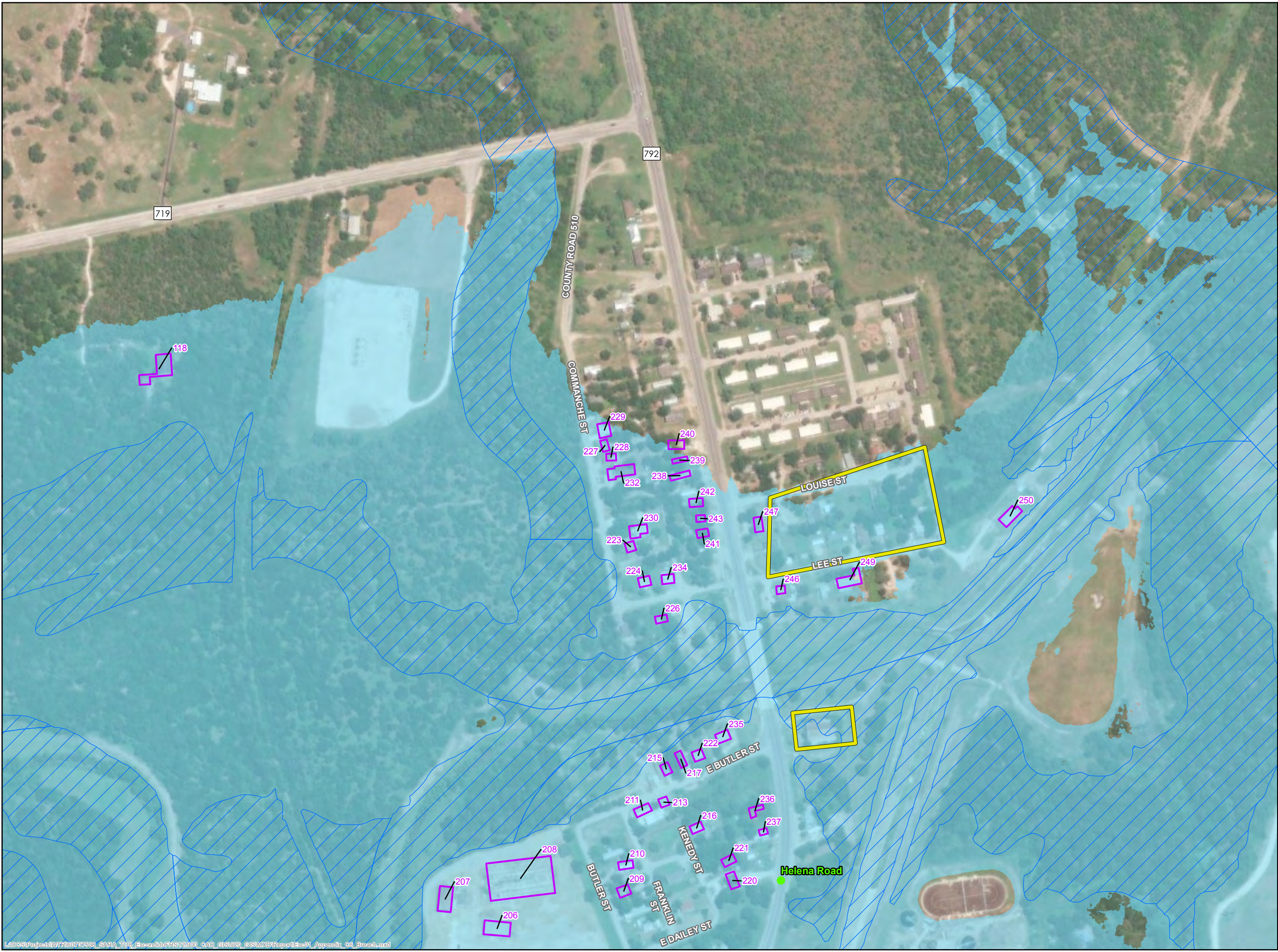
Figure C-6 FRS No. 1 and FRS No. 13 FBH Breach Inundation Map 7 of 13
