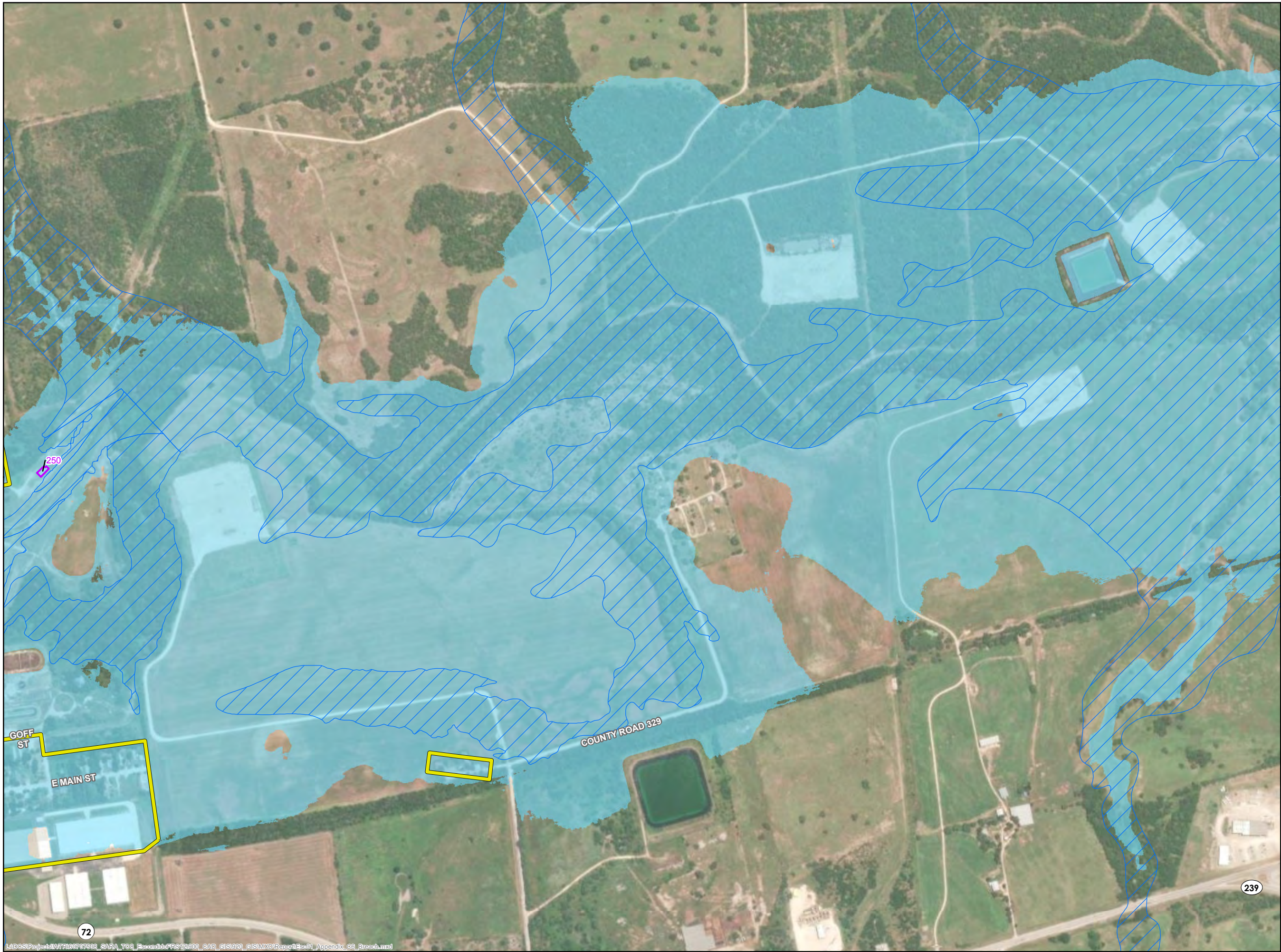
Figure C-6 FRS No. 1 and FRS No. 13 FBH Breach Inundation Map 9 of 13
