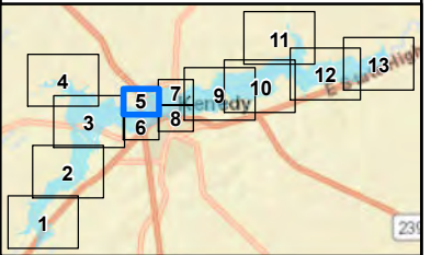
Figure C-6 FRS No. 1 and FRS No. 13 FBH Breach Inundation Map 5 of 13
