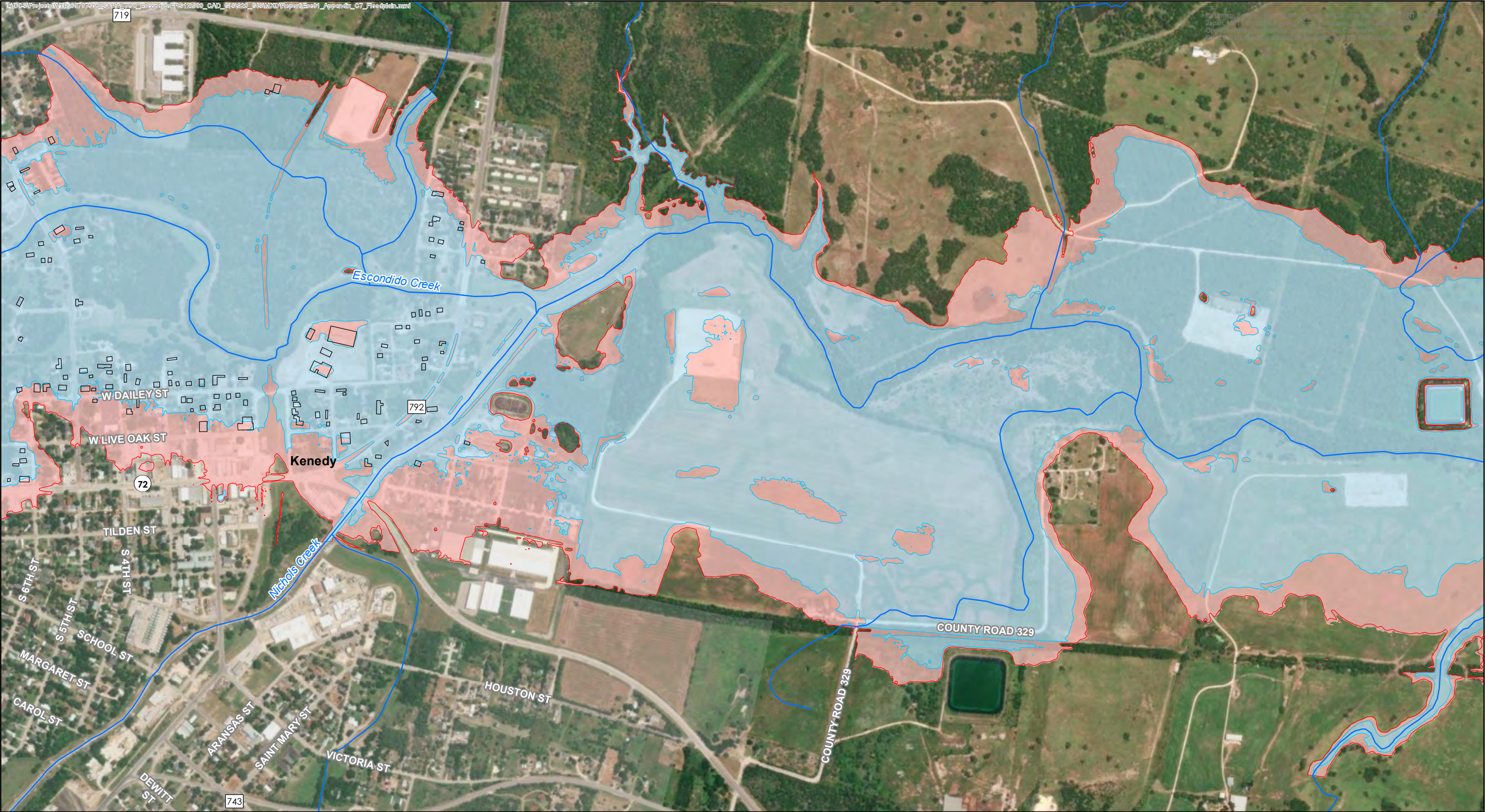
Escondido Creek Watershed Karnes County, Texas Figure C-7 FRS No. 1 Floodplain Map 3 of 6
