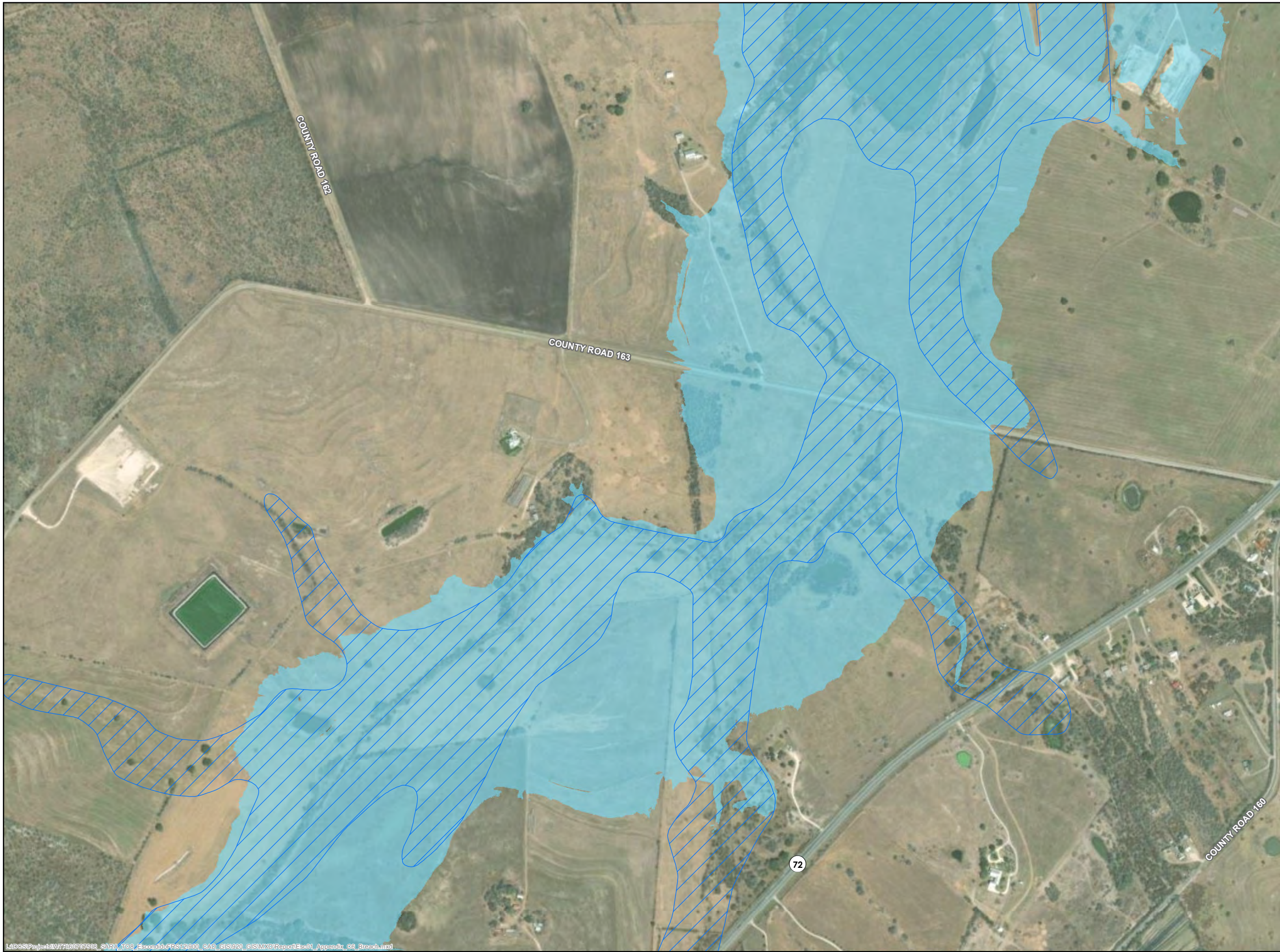
Figure C-6 FRS No. 1 and FRS No. 13 FBH Breach Inundation Map 2 of 13
