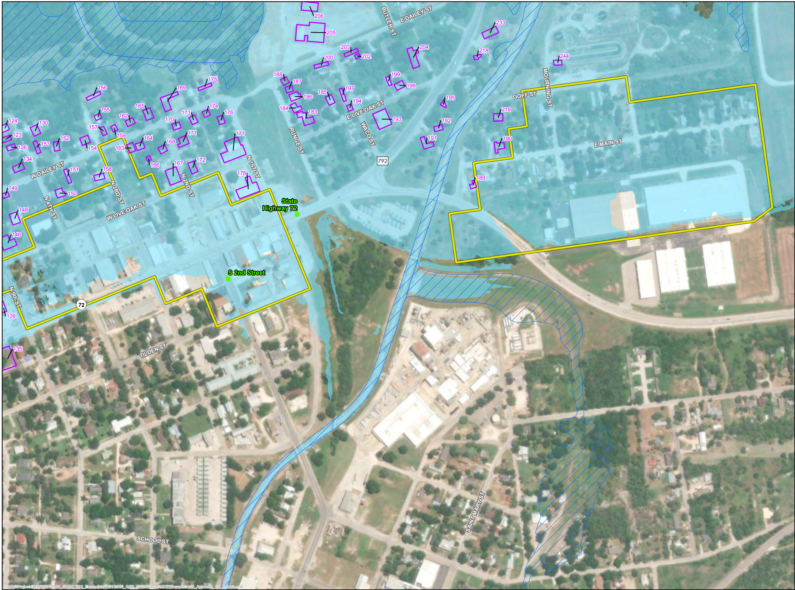
Figure C-6 FRS No. 1 and FRS No. 13 FBH Breach Inundation Map 8 of 13
