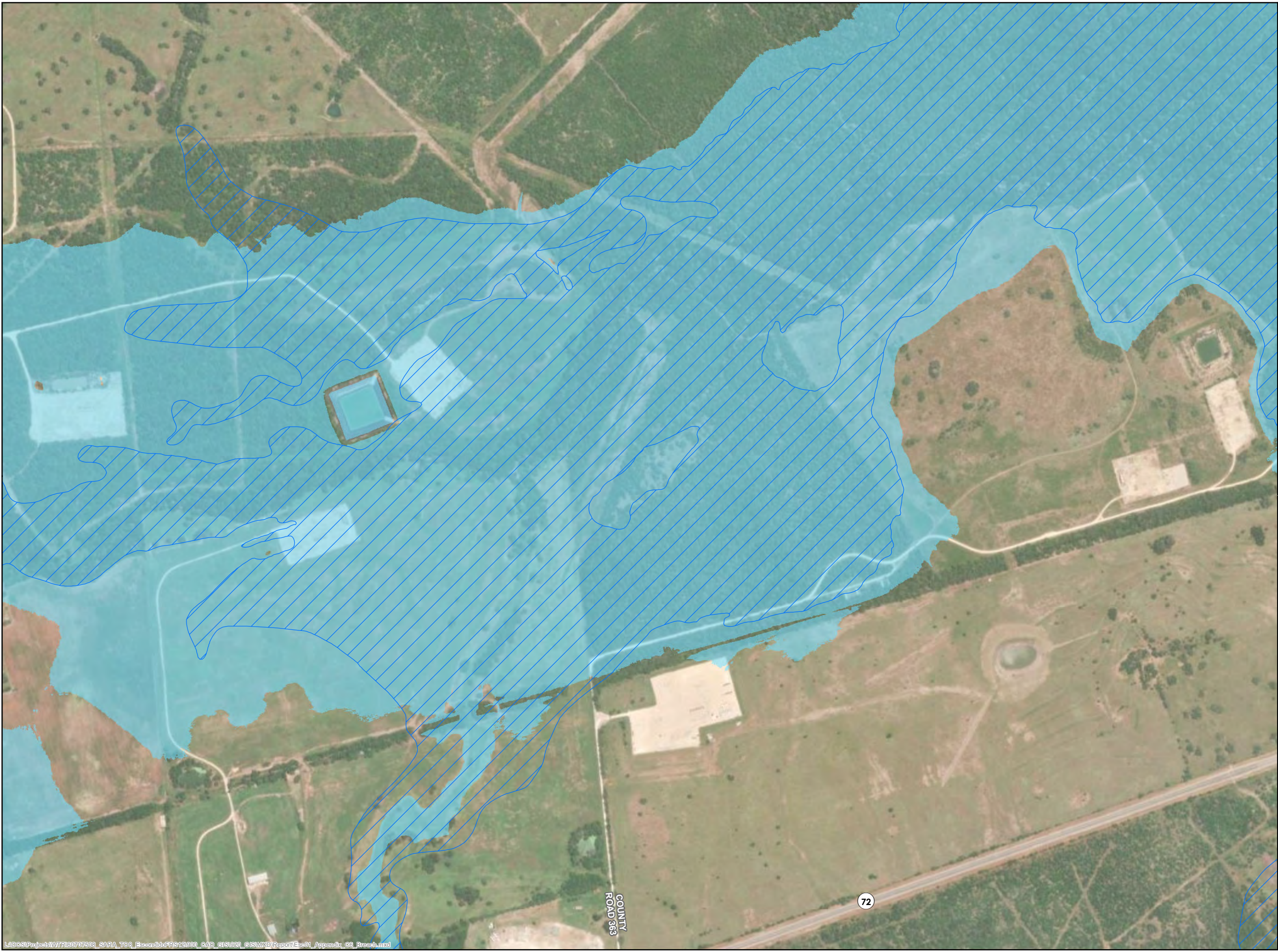
Escondido Creek Watershed FRS No. 1 Karnes County, Texas Figure C-6 FRS No. 1 and FRS No. 13 FBH Breach Inundation Map 10 of 13
