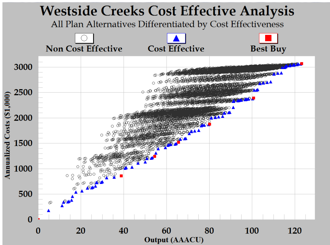
Figure 1. Cost Effective Results
