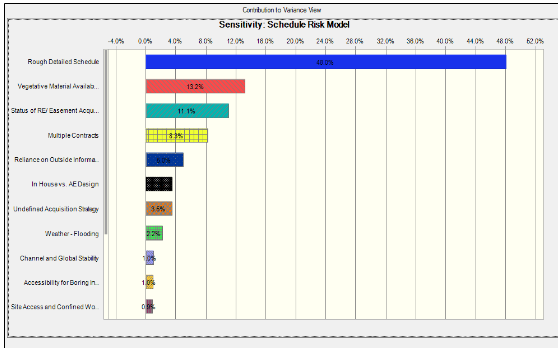
Figure 2. Schedule Sensitivity Analysis
