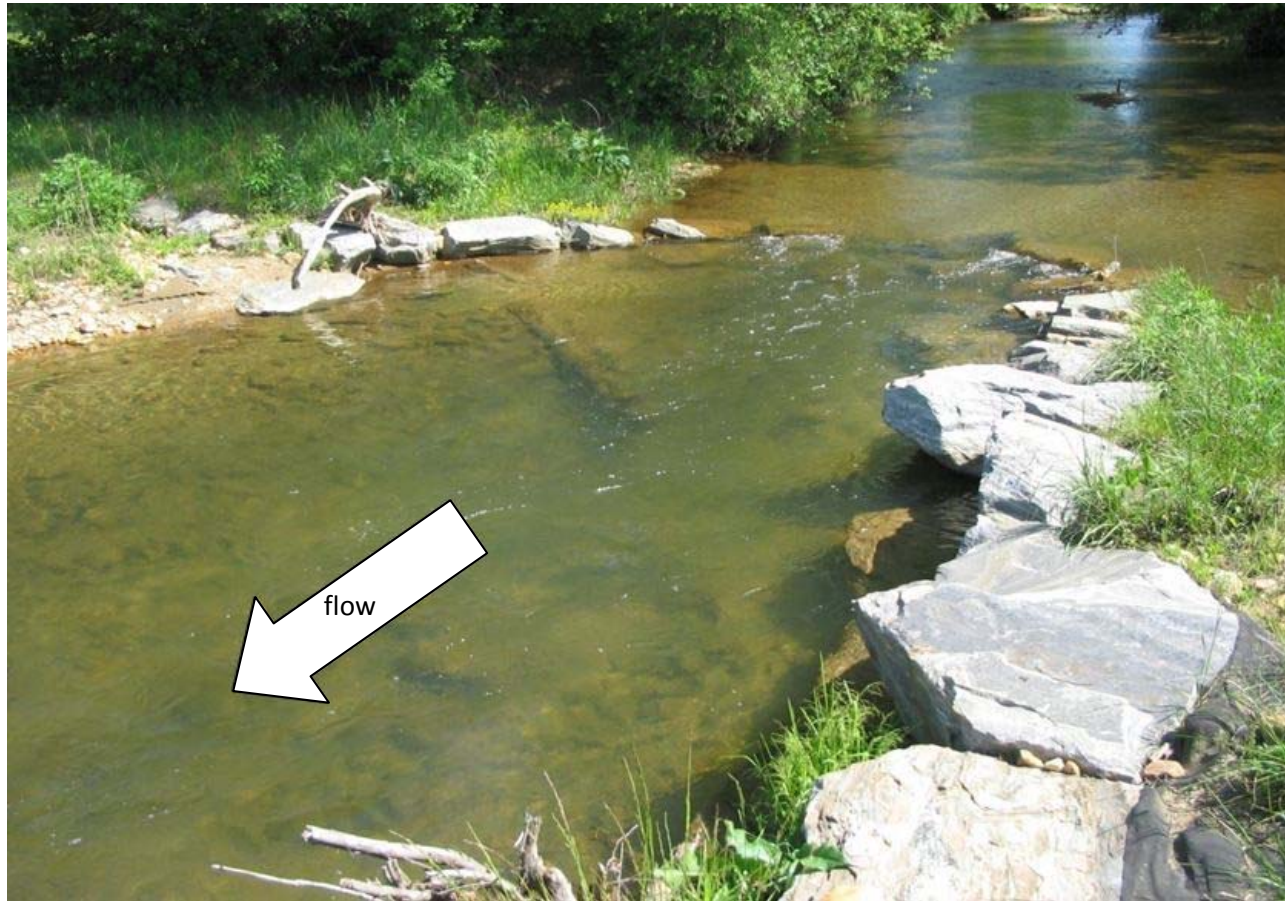
Figure 12. Photo of a Representative Functioning Rock Cross Vane
