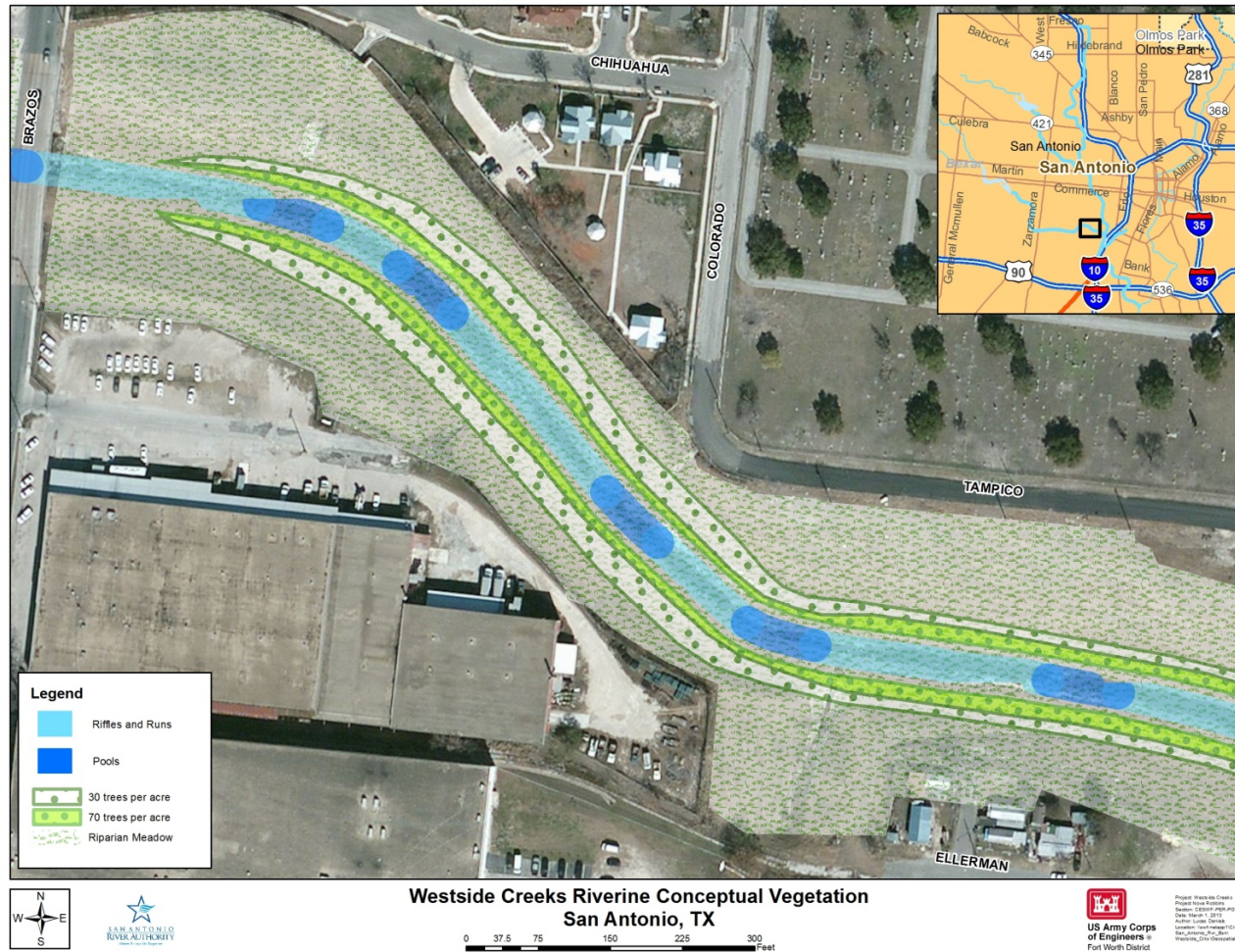
Figure 15. Representative Concept of Maximum Practicable Restoration for the Westside Creeks
