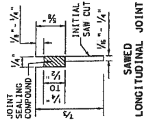
LONGITUDINAL OR TRANSVERSE CONSTRUCTION JOINT
